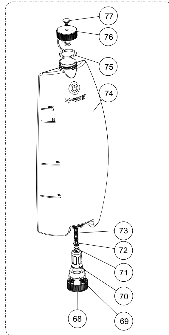
Water tank Assm Unit
