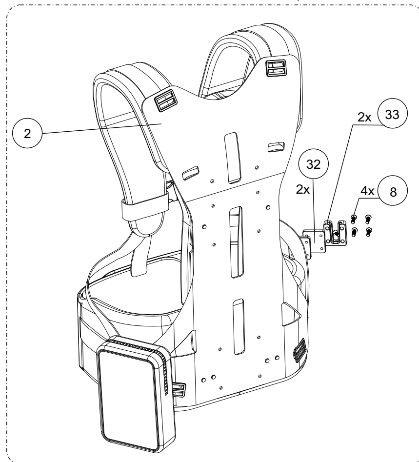
Shoulder harness assm with hook parts
