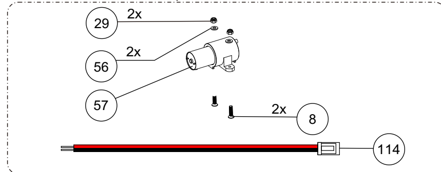
Pump Assm with wires
