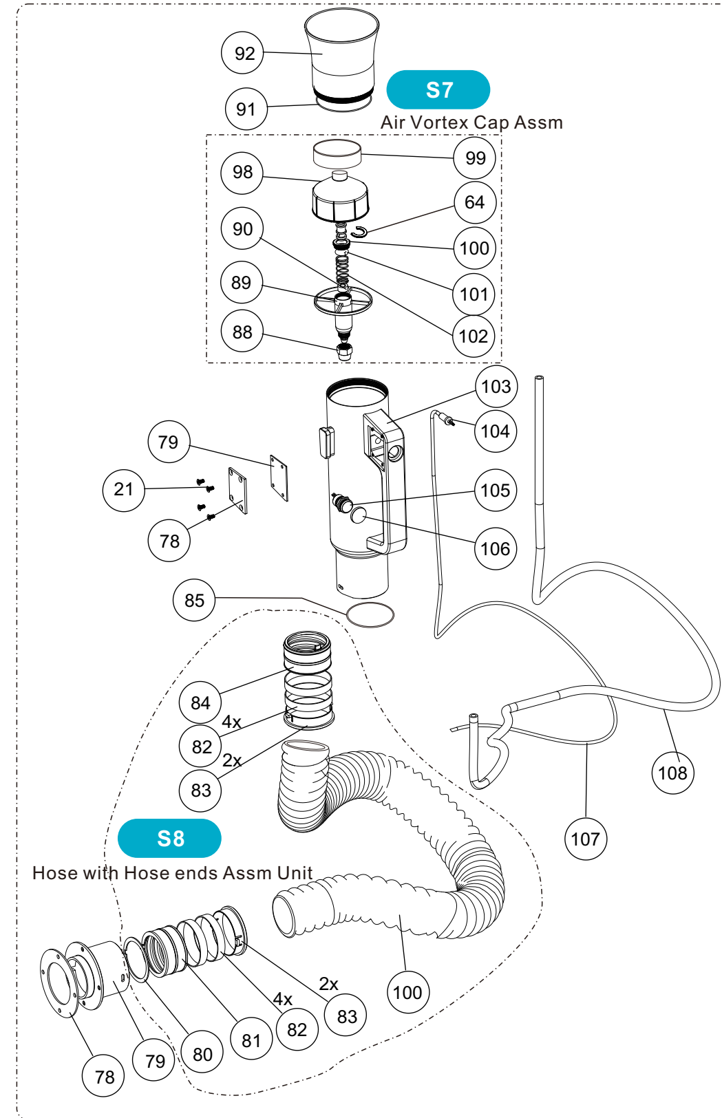
Spray Gun with Hose Assm
