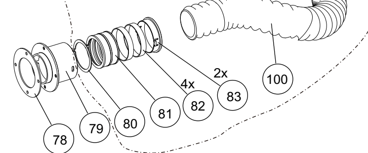
Hose with Hose ends Assm Unit
