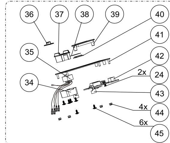
Control panel Assm
