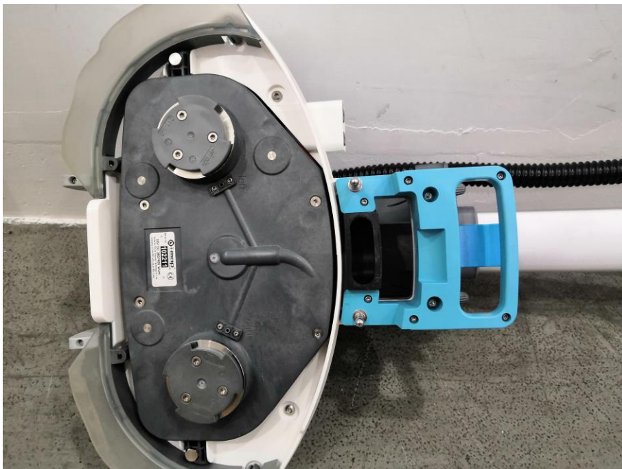
Brush motor internal overview
