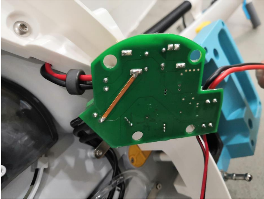
PCB overview
