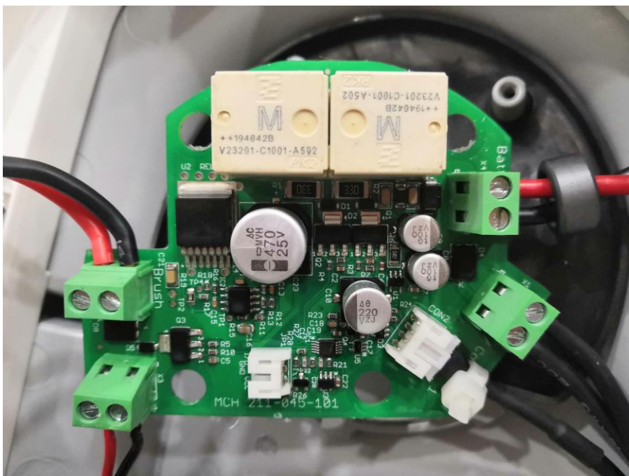
PCB overview
