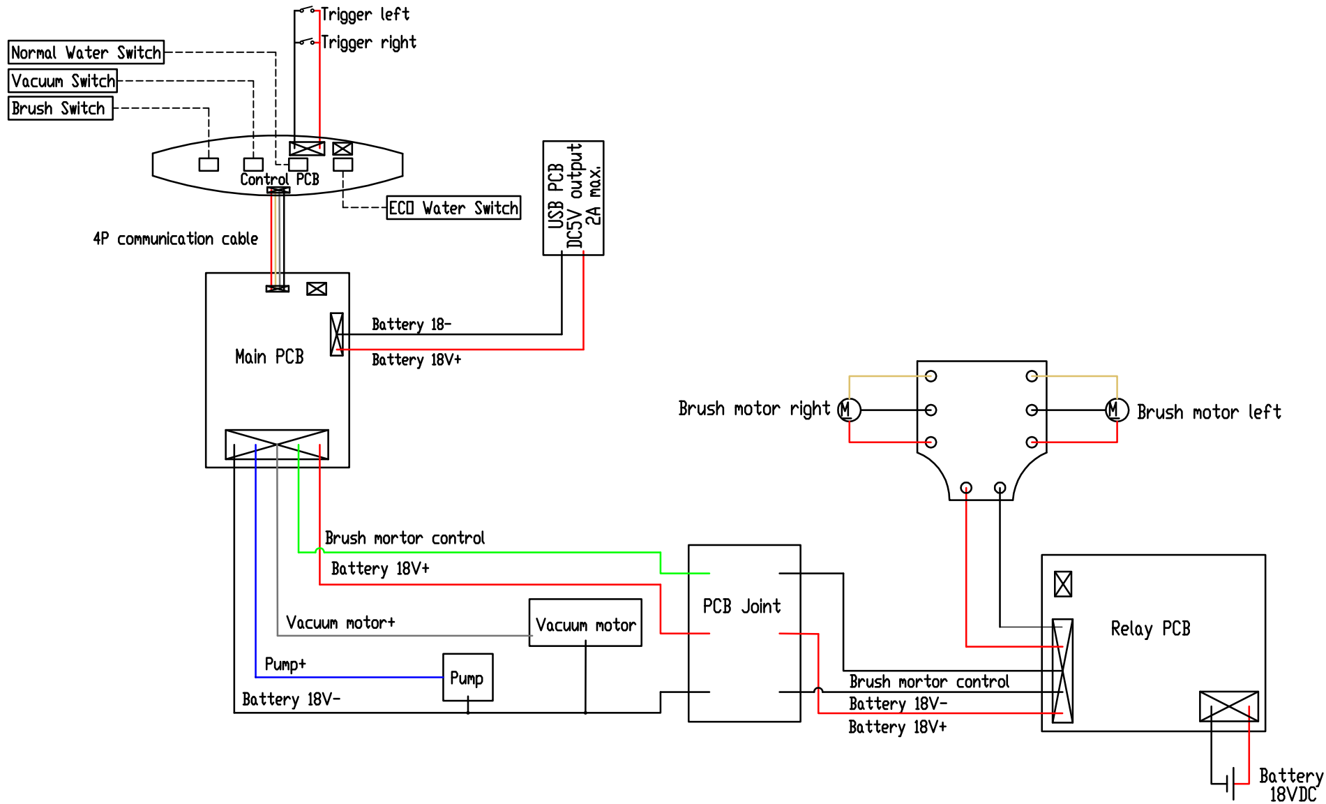
i-mop 36 wiring diagram
